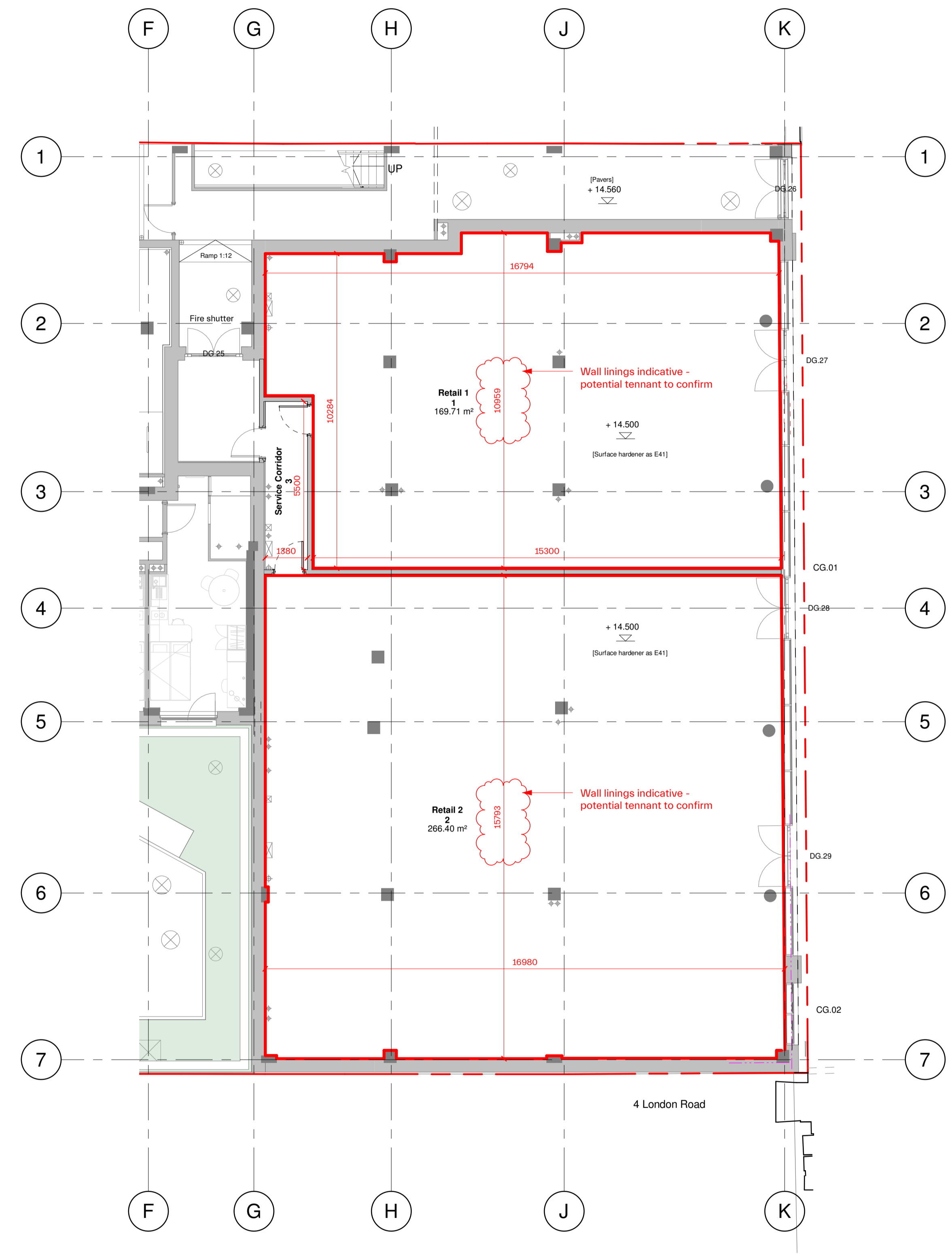
Level 0 Retail Units Demise Plan 1:100
