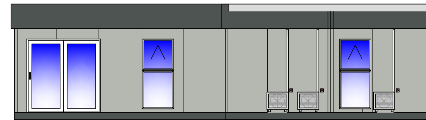
ELEVATION D
